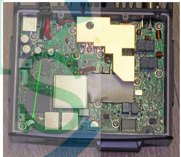
Figure 3 - Main module coin cell location
