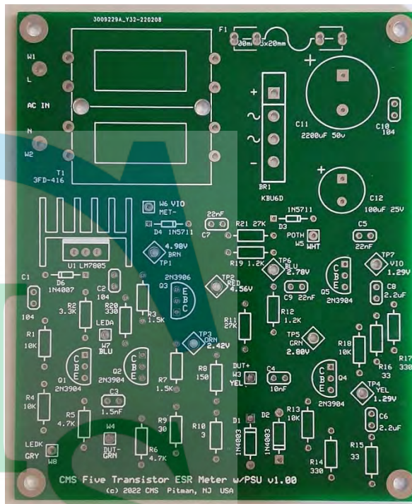
Figure 13 - PCB from JLCPCB
