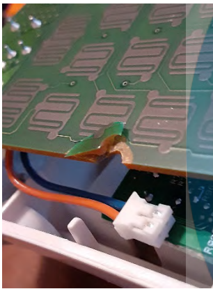
Figure 2 - Delaminated PCB
