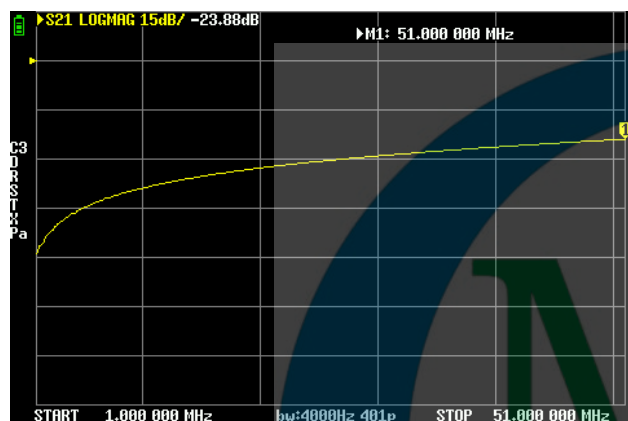
Figure 7 - Insertion loss of B&W model 595 switch
