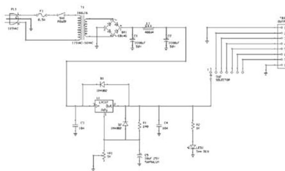
Figure 11 - Controller schematic diagram
