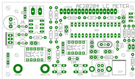
Figure 6 - PCB silk-screen legend
